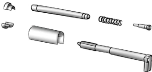
Firing pin
