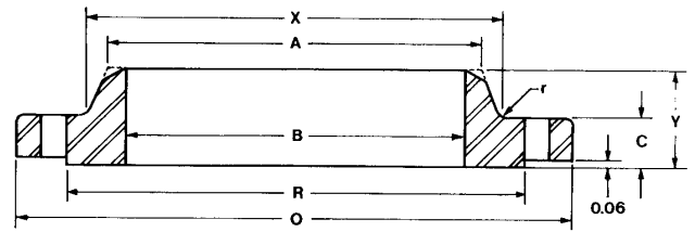
Welding Neck
