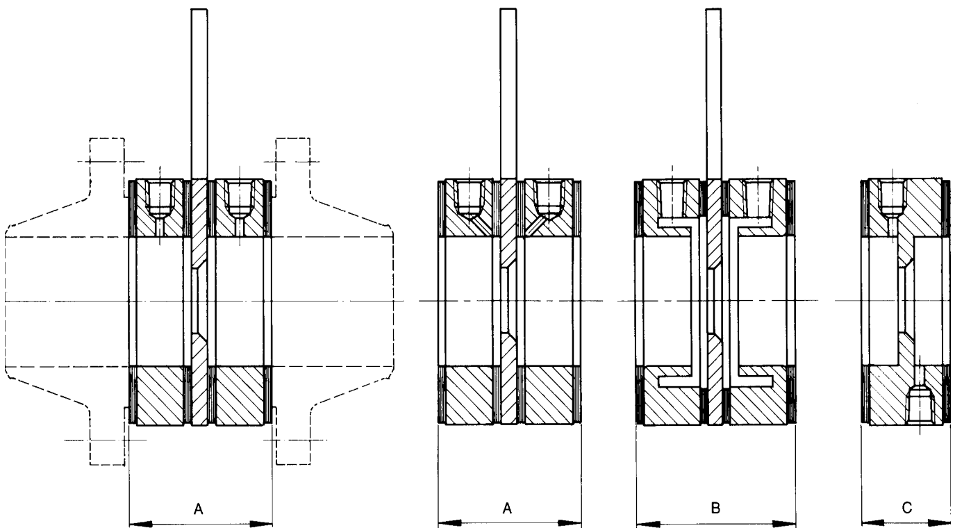
Fig. 1 Flange taps
