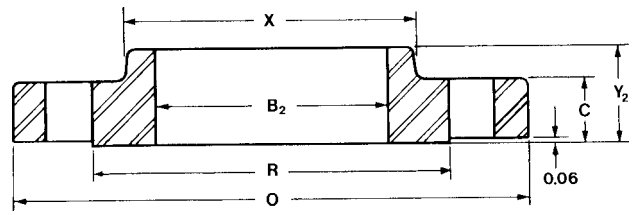
Slip On
