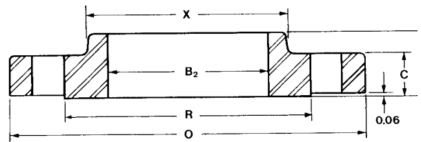
Slip On
