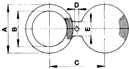
Spectacle plate
