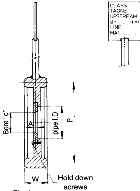
Fig. 1 Octagonal ring to ANSI B16.20 except dim. "W"
