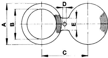
Spectacle plate
