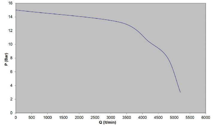
Pump Characteristic Curves PERFORMANCE EXPERIMENT CN10-400
