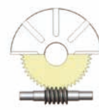
Worm gear drive
