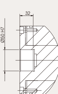
Detail A
