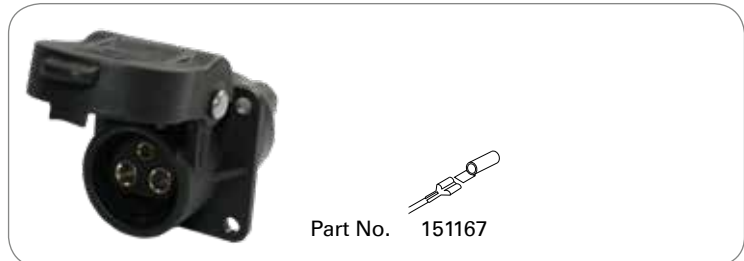
3P/6-24V Plug (DIN 9680)
