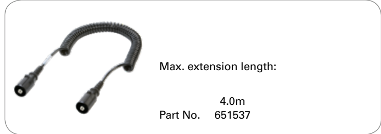
1P/24V Coil (35mm 2 / black)
