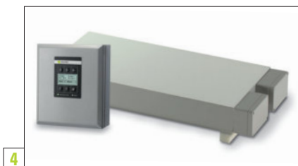
4 ELS Metal Detector Single face ELS metal detectors are installed directly underneath the belt of a conveyor where the depth of conveyed material is shallow ie close to the belt. A typical application is the inspection of sprues to protect auger granulators. ELS can also be used to inspect the quality of plastic components to ensure the core is not broken.
