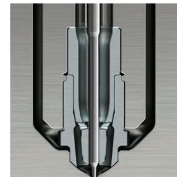
ACCU-VALVE CX (Enhanced color change)
