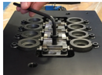
STEP 1 Remove bolt & rectangular washer
