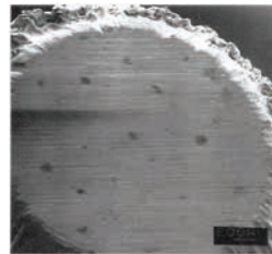
Corrosion and Abrasion damage on valve pin
