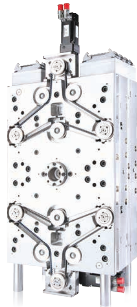
E-Drive synchro plate system
