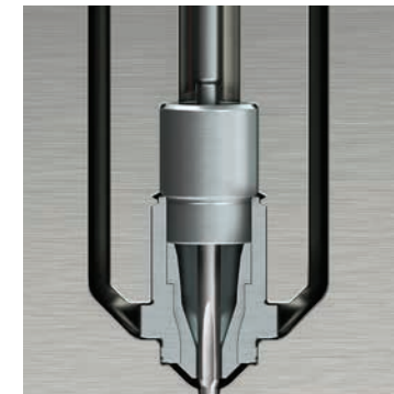
ACCU-VALVE MX (Enhanced fill balance)
