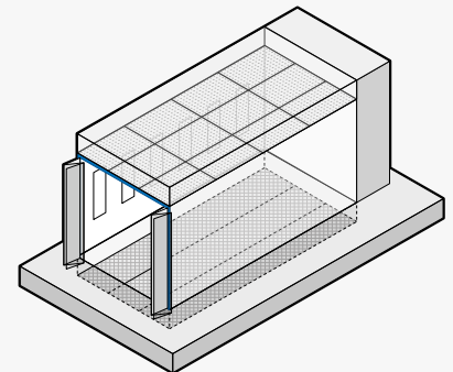
➤ Pressurised spray booth with filtered air inlet plenum and floor extraction
