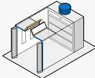
➤ Oblique air flow spray booth with filtered roof air inlet and folding door
