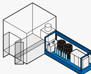
➤ 5-stage skid Hot degreasing, 2 rinses, reverse osmosis + passivating rinse
