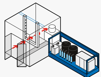
➤ 5-stage skid with automatic washing portal for automatic and manual washing in the same booth
