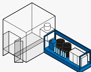
➤ 4-stage skid Hot degreasing, 2 rinses + reverse osmosis rinse
