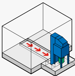
➤ Semi-automatic recovery with transversal screw with localised civil works
