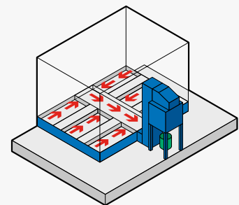
➤ Automatic above floor recovery without civil works, with raised work platform
