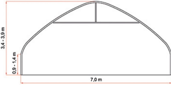
Tunel 7,0m
