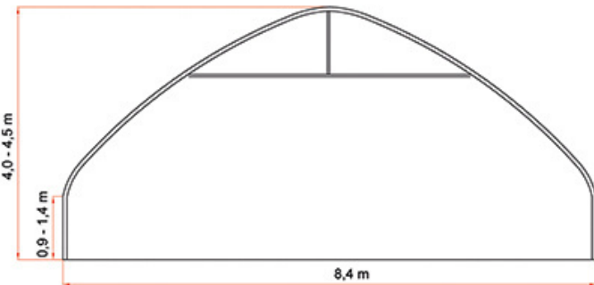
Tunel 8,4m
