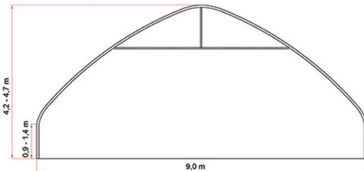
Tunel 9,0m
