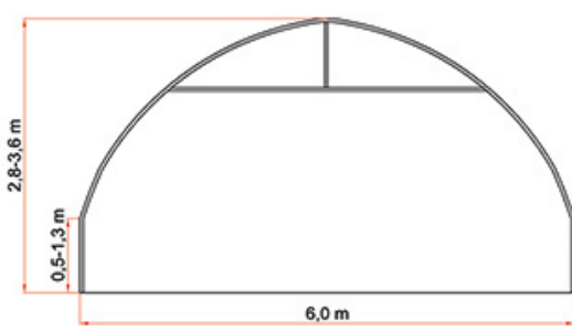
Tunel 6,0m
