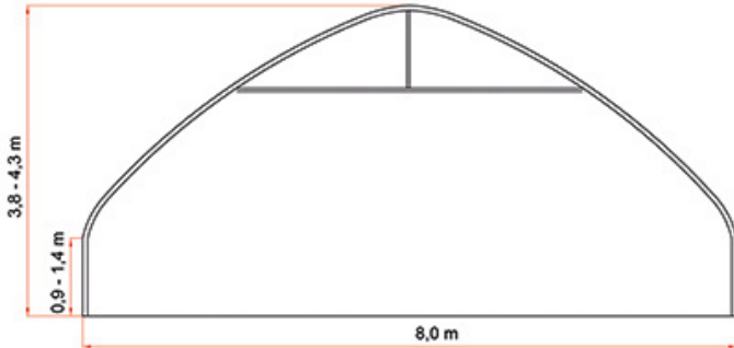
Tunel 8,0m
