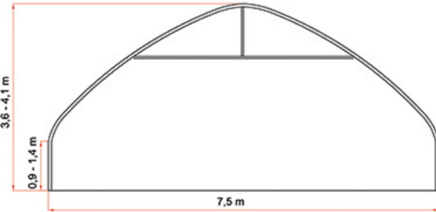
Tunel 7,5m
